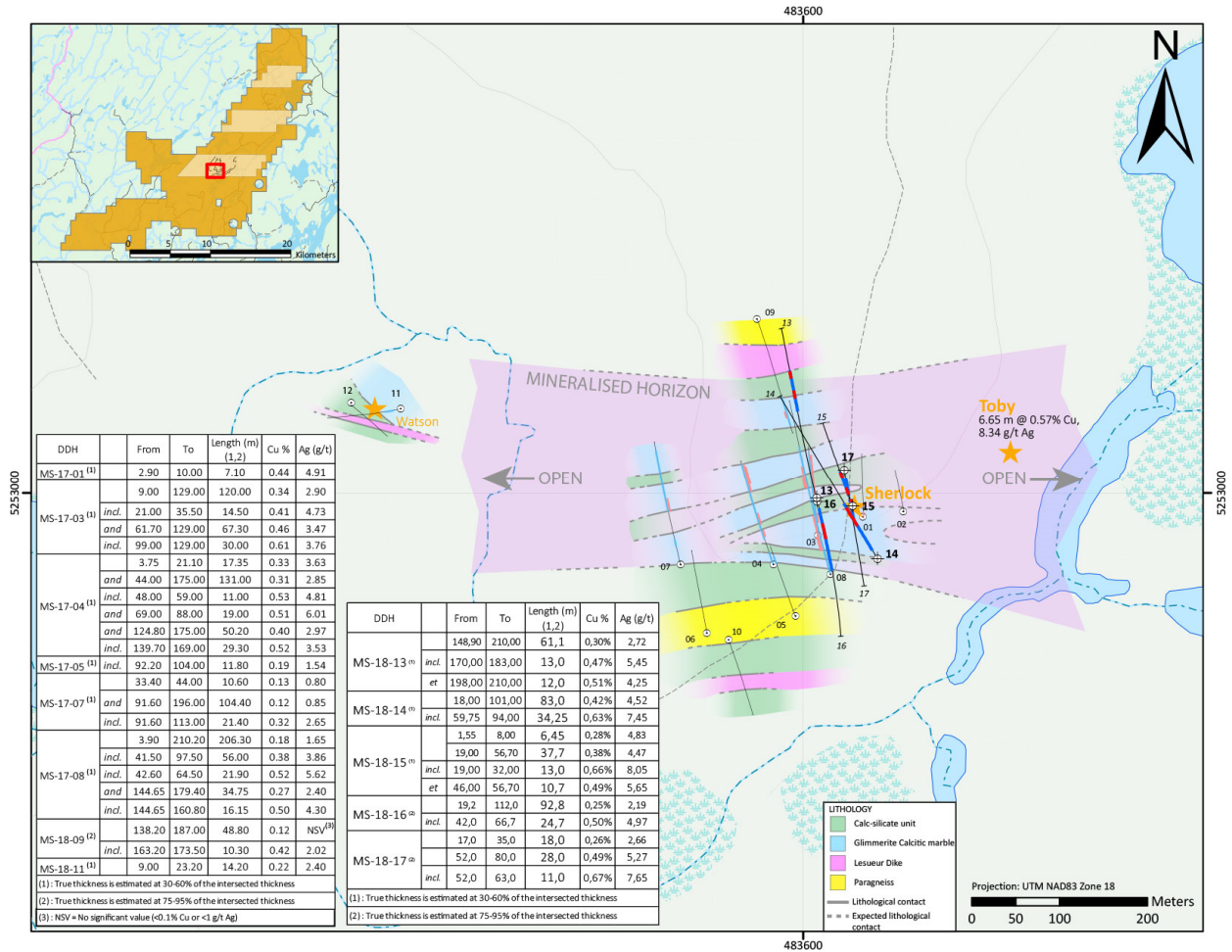
Figure 1: Location of the first 5 drill holes of the 2018 program and their mineralized intersections, Full size map can be viewed here ,
